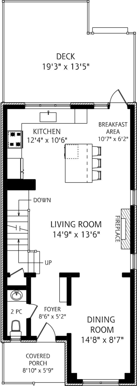
MAIN FLOOR
