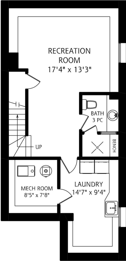
LOWER LEVEL
